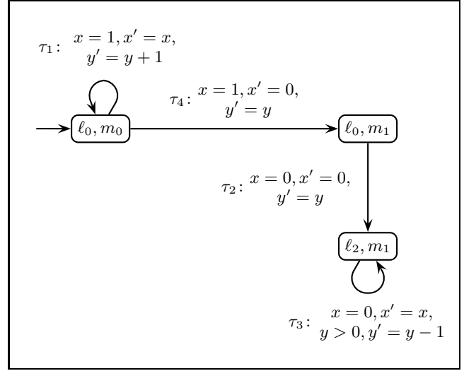
Figure 6: Control-flow graph for the parallel composition of processes P_1 and P_2 in ANY-DOWN.
