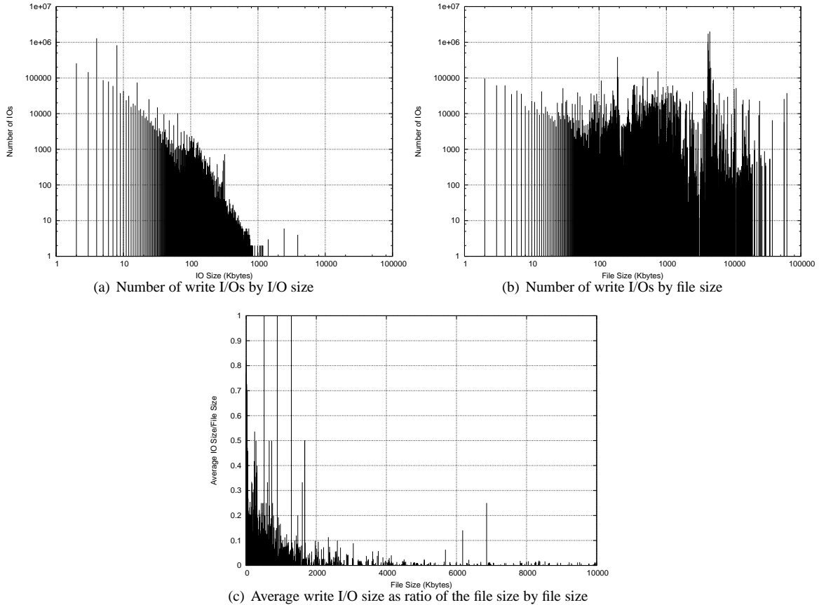
Figure 4: Characterization of write I/Os from trace-driven experiments.
