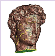
closed 1-chain
