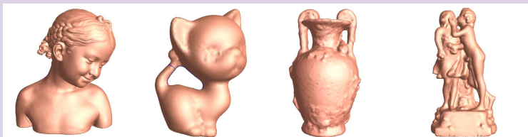
Figure: Surface topological classification
