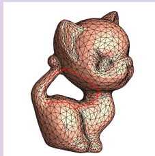
closed, non-exact 1-chain
