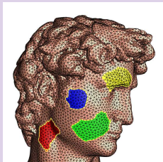
exact 1-chain
