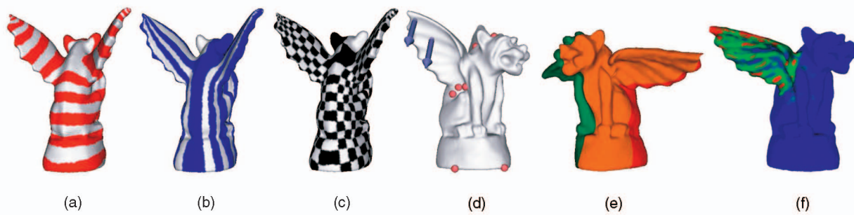
Fig. 10. (a), (b), and (c) The global conformal parameterization of the gargoyle model. (d) User’s applied forces and specified position constraints. (e) The deformation of the gargoyle’s wings (different parametric patches are shown in different colors). (f) The stress distribution after deformation.
