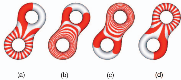
Fig. 2. The harmonic 1-forms \{\omega_1, \omega_2, \omega_3, \omega_4\} computed by (1). (a) \omega_1 dual to a_1 , (b) \omega_2 dual to b_1 , (c) \omega_3 dual to a_2 , and (d) \omega_4 dual to b_2 .
