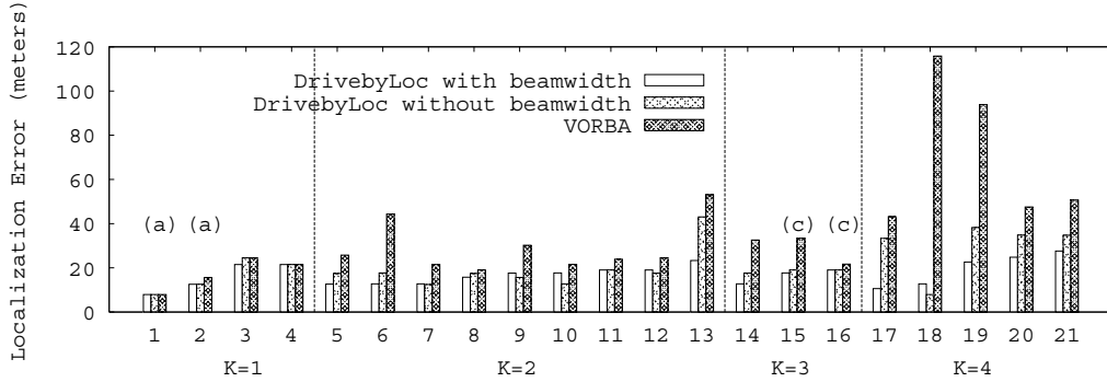
Fig. 8. Comparison of DrivebyLoc and VORBA.
