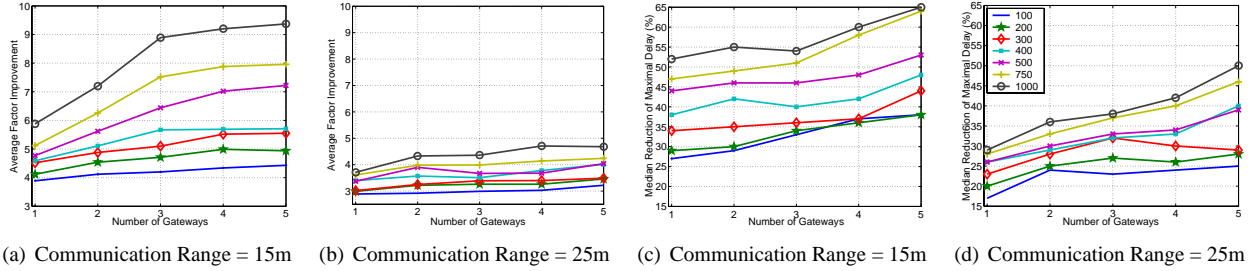
Figure 1. (a,b) Relative effectiveness for delay reduction using heuristic vs. pseudo random gateway placement. (c,d) Median delay improvement optimized using LB heuristic over the greedy approach.
