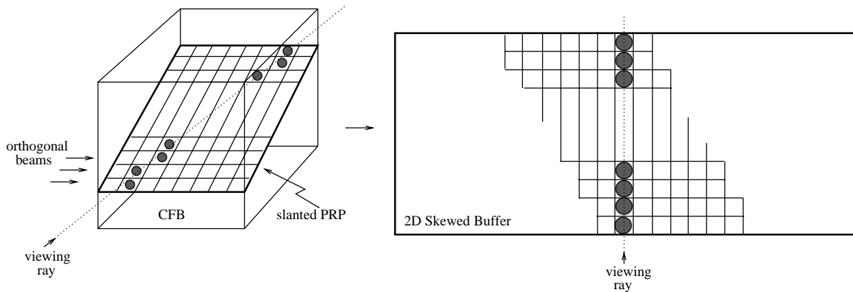
Fig. 1.2. Transfer of the projection ray plane to 2D skewed buffer
