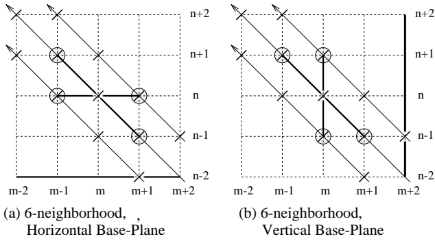
Figure 8: 6-neighborhood Gradient.
