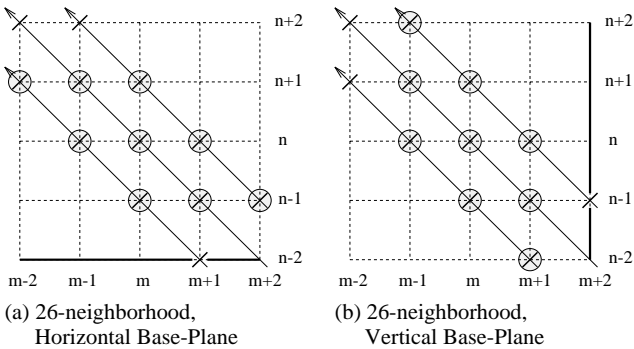
Figure 9: 26-neighborhood Gradient.
